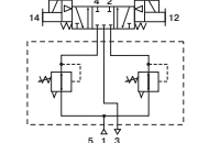
Independent Dual Port Regulator with 4-Way, 3-Position Double Solenoid Valve
