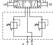
Independent Dual Port Regulator with 4-Way, 3-Position Double Solenoid Valve
