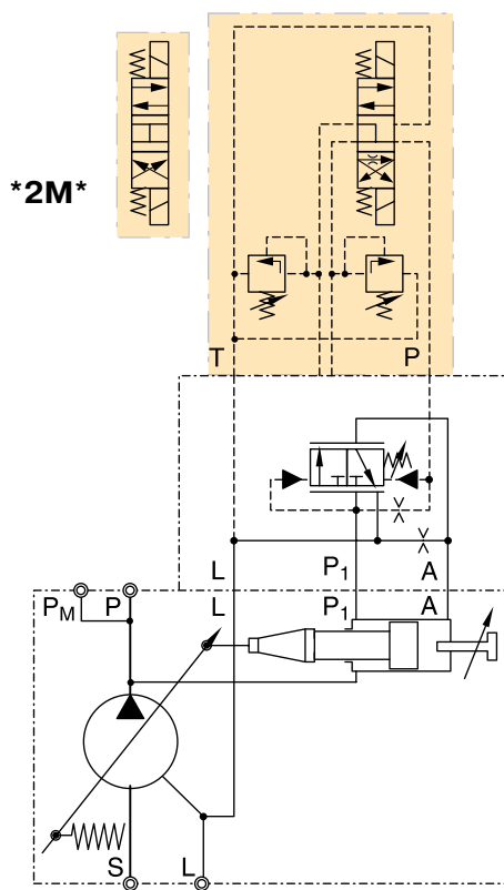
Schaltplan PVAC2M*/PVAC2E*
