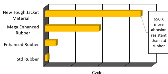
Hydraulic Tough Jacket Hose vs. Competitors Full Weight ISO 6945
