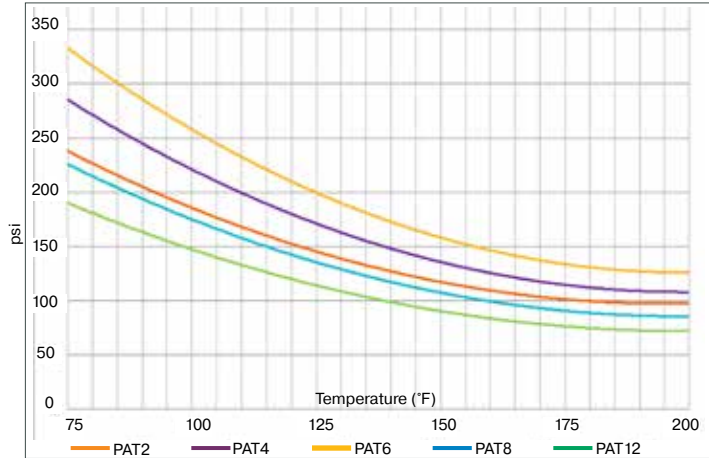
Nylon Tubing (Series PAT) Maximum Working Pressure (psi)
